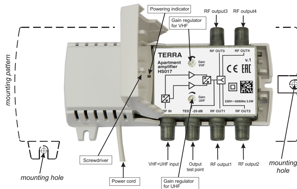
Figure 1. External view of the amplifier and operating controls
