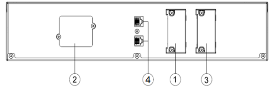
BPSE36V45ART2U, BPSE72V45ART2U
